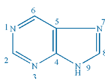
Purine
