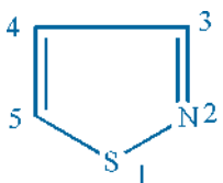
Isotiazole
