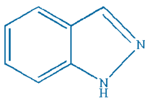
Indazole
