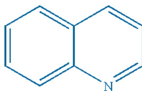
Quinoline
