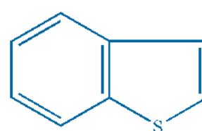
Benzothiophene
