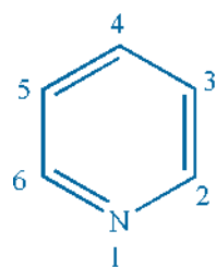
Pyridine
