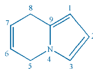
Indolizine
