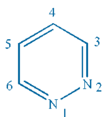
Pyridazine
