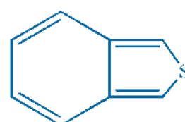
Isobenzothiophene
