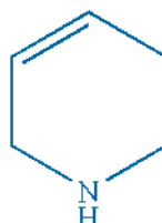
Tetrahydropyridine
