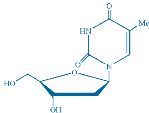
2-Deoxythymidine
