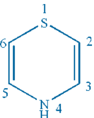
1,4-Thiazine
