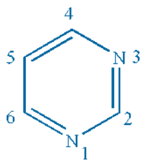
Pyrimidine
