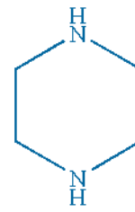
Piperazine
