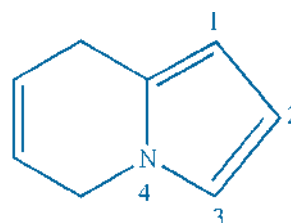
Indolizine
