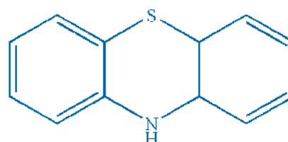
Phenothiazine
