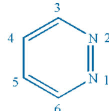
Pyridazine
