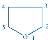
Tetrahydrofuran
