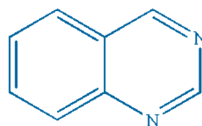
Quinazoline
