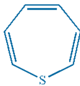
Thiepine
