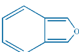
Isobenzofuran
