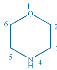
Morpholine
