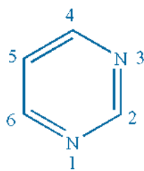
Pyrimidine
