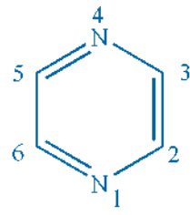
Pyrazine
