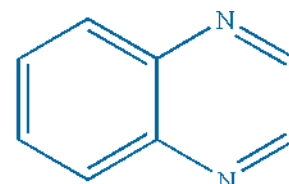
Quinoxaline
