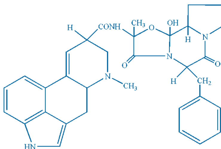
Ergotamine
