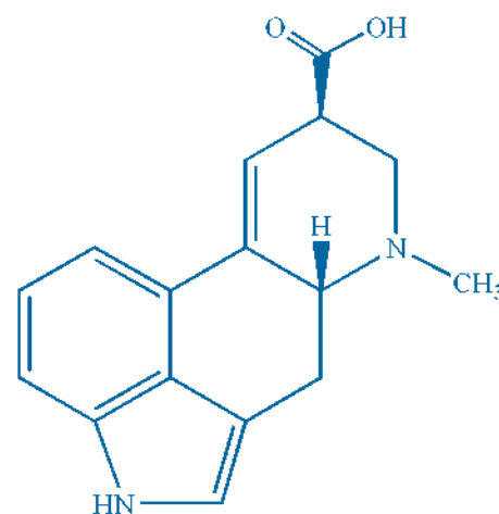
Lysergic acid
