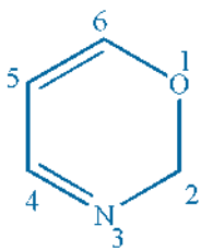
1,3-Oxazine
