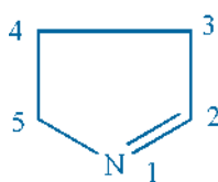
\Delta^1 -Pyrroline
