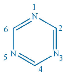
1,3,5-Triazine
