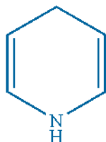
Dihydropyridine
