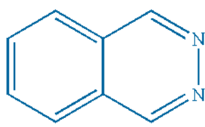
Phthalazine
