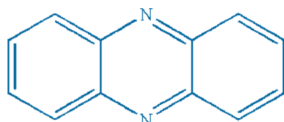
Phenazine
