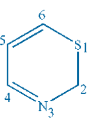
1,3-Thiazine
