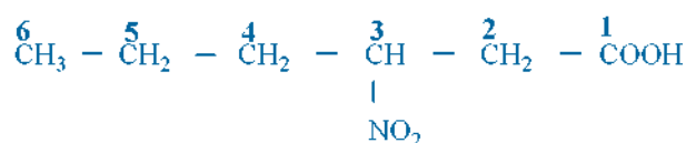
3-Nitrohexanoic acid
