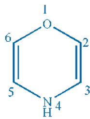
1,4-Oxazine
