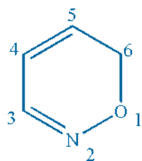
1,2-Oxazine
