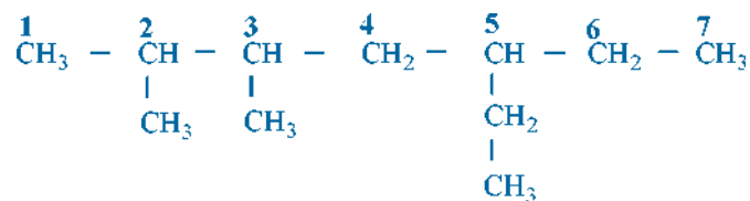
2,3-Dimethyl-5-ethyl heptane (wrong)
