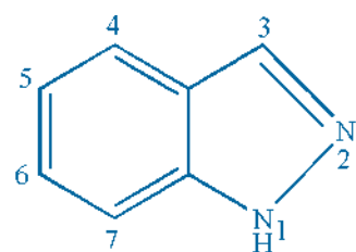
Indazole
