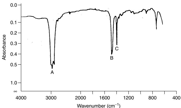
Figure 4.1 Infrared spectrum of nonane ( \text{C}_9\text{H}_{20} ) (cf. SAQ 4.1). From Stuart, B., Modern Infrared Spectroscopy , ACOL Series, Wiley, Chichester, UK, 1996. © University of Greenwich, and reproduced by permission of the University of Greenwich.
