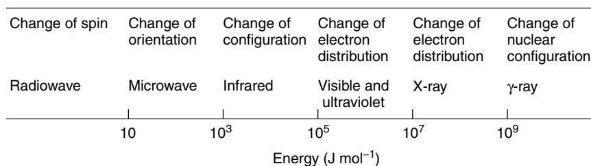
Figure 1.1 Regions of the electromagnetic spectrum. From Stuart, B., Biological Applications of Infrared Spectroscopy , ACOL Series, Wiley, Chichester, UK, 1997. © University of Greenwich, and reproduced by permission of the University of Greenwich.
