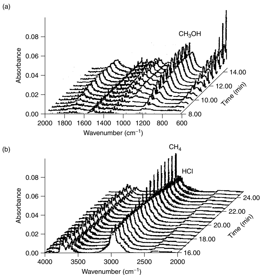
Figure 6.20 Evolution of gases as a function of time from a blend of PMMA and \text{Fe(III)} chloride, where a time of 8 min corresponds to a temperature of 160°C (ramp rate of 20°C \text{min}^{-1} ). Reprinted from Polym. Degrad. Stabil. , 66 , Wilkie, C. A., 'TGA/FTIR: An extremely useful technique for studying polymer degradation', 301–306, Copyright (1999), with permission from Elsevier.
